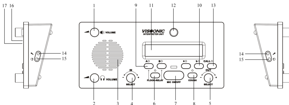
Figure 4.1 VIS-INT64
