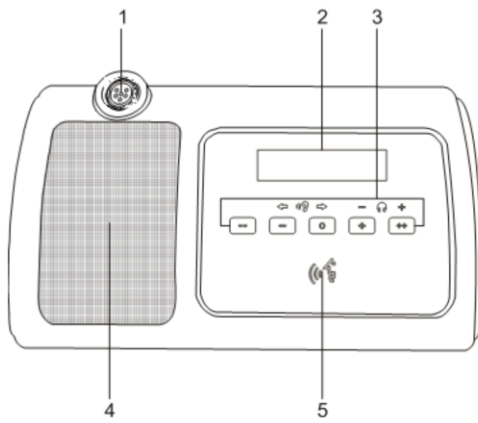
Figure 3.1.1.1 Top view of wired units VIS-DCC/DCC/DVC/DVD/DVCIC/DVDIC-T
