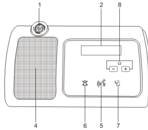
VIS-DVC-T/VIS-DVCIC-T
