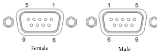
Figure 2.1.3.7.2 Pin descriptions of the CONTROL interface
