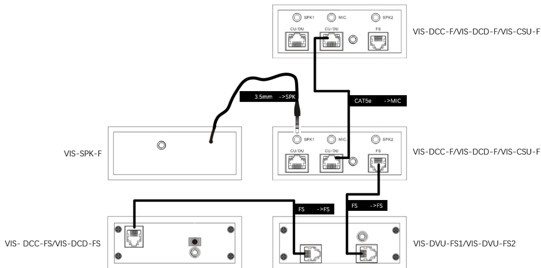
Figure 3.5.3 Connection of VIS-DCC/DCD/CSU/DVU/SPK-F/FS/FS1/FS2
